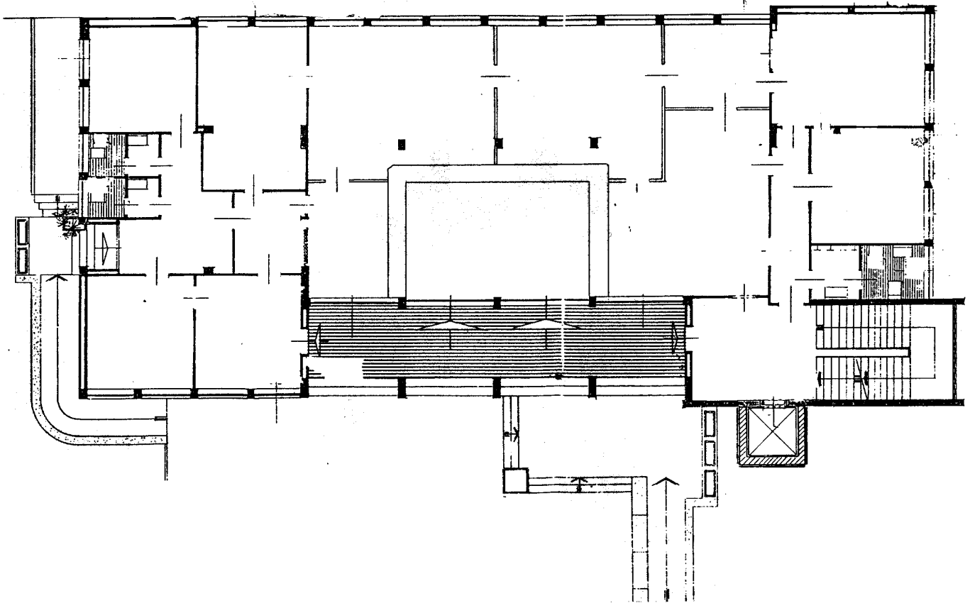
PIANO TERRA
