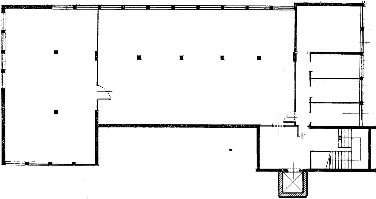
PIANO CANTINA
